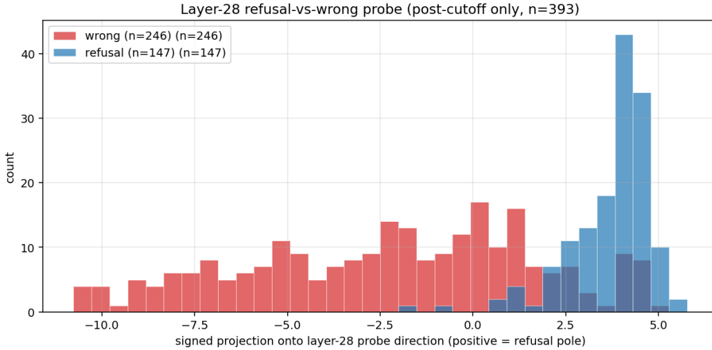
Figure 11: Score histogram: the signed projection of each item’s layer-28 hidden state onto the recovered refusal direction, on the within-post subset ( n = 393 ). Refusals concentrate at large positive projections; wrongs near zero or negative.
