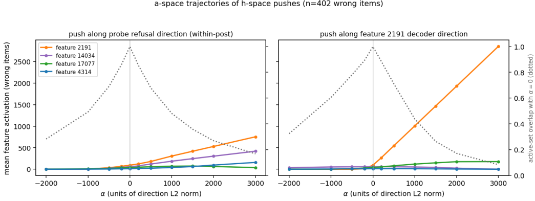
Figure 13: a-space trajectories of h-space pushes ( n = 402 wrong items, pre-norm residuals). Solid lines: mean activation of four ensemble features as the state is pushed along the Section 6.2 refusal direction (left) or feature 2191’s decoder direction (right); dotted: mean overlap (Jaccard) of the active feature set with the unperturbed code. The probe push recruits the register broadly; the 2191 push concentrates on the opener and crowds out the hedge.
