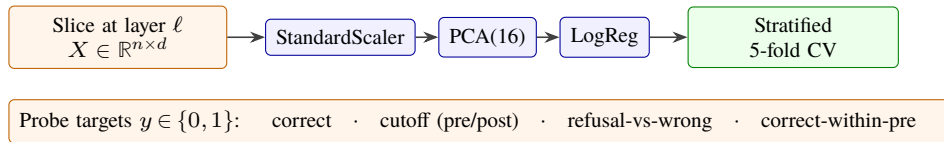
Figure 7: Per-layer linear-probe pipeline. At each layer \ell , the n \times d matrix of captured hidden states is passed through StandardScaler \rightarrow PCA(16) \rightarrow logistic regression and evaluated with stratified 5-fold CV, separately for each binary target.
