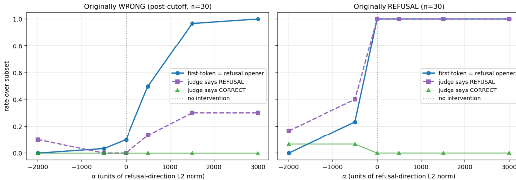
Figure 10: Causal intervention: rate over each subset as a function of \alpha . Solid blue: fraction of generations whose first generated token matches a refusal opener ( \{\text{as, As, as, 作为, 作为, 作为一个}\} ). Dashed purple: fraction whose full judge label is REFUSAL. Light green: fraction labeled CORRECT (drops at high |\alpha| on the refusal subset: intervention can also break originally correct refusals into confabulations). The first-token measure changes monotonically and saturates near \alpha = \pm 1500 ; the full-judge measure changes more slowly because of autoregressive continuation dynamics.
