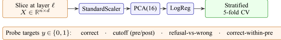
Figure 3: Per-layer linear-probe pipeline. At each layer \ell , the n \times d matrix of captured hidden states is passed through StandardScaler \rightarrow PCA(16) \rightarrow logistic regression and evaluated with stratified 5-fold CV, separately for each binary target.
