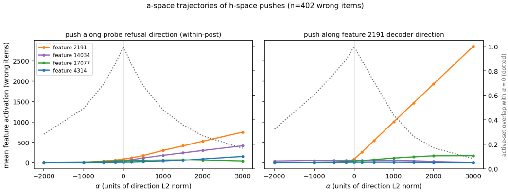
Figure 13: a-space trajectories of h-space pushes ( n = 402 wrong items, pre-norm residuals). Solid lines: mean activation of four ensemble features as the state is pushed along the Section 6.2 refusal direction (left) or feature 2191’s decoder direction (right); dotted: mean overlap (Jaccard) of the active feature set with the unperturbed code. The probe push recruits the register broadly; the 2191 push concentrates on the opener and crowds out the hedge.
