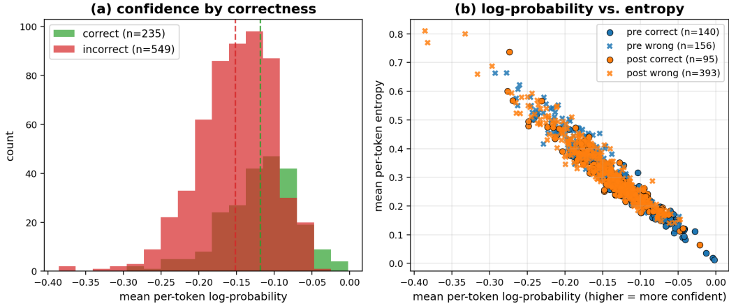
Figure 4: Text-level confidence. (a) Histogram of per-item mean per-token log-probability under greedy decoding, split by judge correctness label: the two distributions overlap substantially, their means differing by \approx 0.05 nats. (b) Per-item mean log-probability vs. mean entropy, colored by cutoff class, marker by correctness. Pre/post-cutoff items occupy distinguishable regions but with heavy overlap, especially among confident wrongs.
