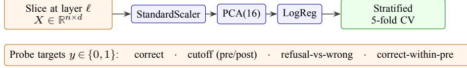
Figure 2: Per-layer linear-probe pipeline. At each layer \ell , the n \times d matrix of captured hidden states is passed through StandardScaler \rightarrow PCA(16) \rightarrow logistic regression and evaluated with stratified 5-fold CV, separately for each binary target.
