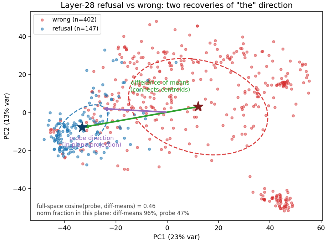
Figure 9: Two recoveries of “the” refusal direction, in the top two principal components of the layer-28 refusal+wrong hidden states ( n = 549 ). Stars: class centroids; dashed curves: per-class 1\sigma covariance ellipses. The class-mean difference (green) connects the centroids and lies almost entirely (96% of its norm) in this top-variance plane; the probe direction (purple, in-plane projection) keeps only 47% of its norm here, the rest living in lower-variance axes where the classes separate cleanly. Full-space cosine between the two: 0.46.
