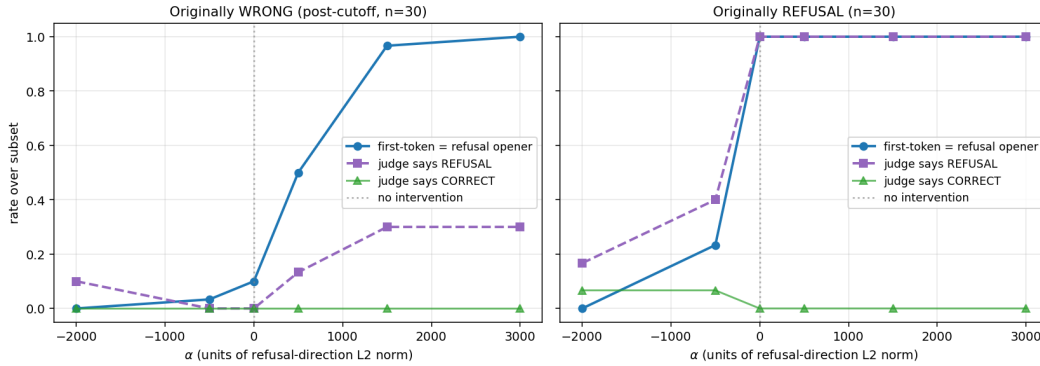
Figure 9: Causal intervention: rate over each subset as a function of \alpha . Solid blue: fraction of generations whose first generated token matches a refusal opener ( \{\text{as, As, 作为, 作为一个}\} ). Dashed purple: fraction whose full judge label is REFUSAL. Light green: fraction labeled CORRECT (drops at high |\alpha| on the refusal subset: intervention can also break originally correct refusals into confabulations). The first-token measure changes monotonically and saturates near \alpha = \pm 1500 ; the full-judge measure changes more slowly because of autoregressive continuation dynamics.
