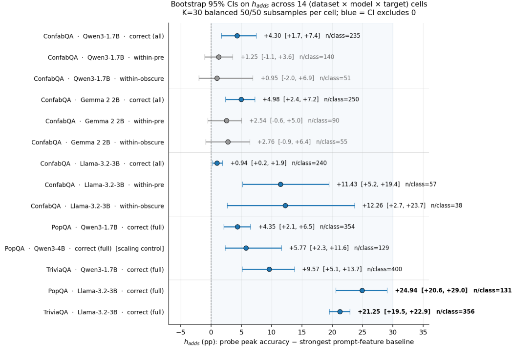
Figure 13: Bootstrap 95% CIs on h_{\text{adds}} across 14 (dataset, model, target) cells. K = 30 balanced 50/50 subsamples per cell; blue = CI excludes 0. The bottom two rows are the headline positive finding: Llama 3.2 3B on PopQA / TriviaQA recovers +21–+25 pp over the strongest prompt-feature baseline, where Qwen3-1.7B and Qwen3-4B on the same data recover +4–+10 pp. The Qwen3-4B row labeled “scaling control” rules out parameter count as the dominant driver of the cross-model gap.
