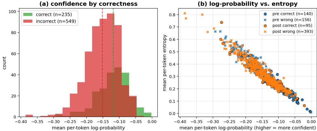
Figure 5: Text-level confidence. (a) Histogram of per-item mean per-token log-probability under greedy decoding, split by judge correctness label: the two distributions overlap substantially, their means differing by \approx 0.05 nats. (b) Per-item mean log-probability vs. mean entropy, colored by cutoff class, marker by correctness. Pre/post-cutoff items occupy distinguishable regions but with heavy overlap, especially among confident wrongs.
