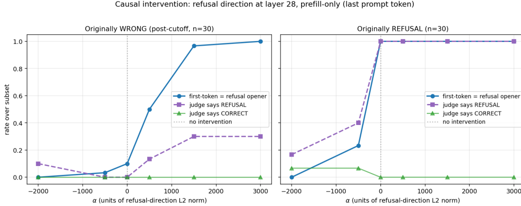
Figure 9: Causal intervention: rate over each subset as a function of \alpha . Solid blue: fraction of generations whose first generated token matches a refusal opener ( \{ \text{as, As, as, 作为, ...} \} ). Dashed purple: fraction whose full judge label is REFUSAL. Light green: fraction labeled CORRECT (drops at high |\alpha| on the refusal subset: intervention can also break originally correct refusals into confabulations). The first-token measure changes monotonically and saturates near \alpha = \pm 1500 ; the full-judge measure changes more slowly because of autoregressive continuation dynamics.
