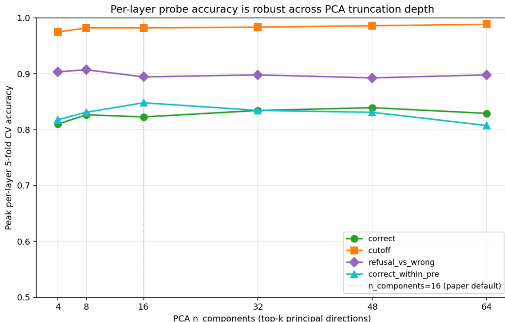
Figure 16: Peak per-layer probe accuracy as a function of PCA n_{\text{components}} for each of the main probe targets. The paper default ( n = 16 ) is marked. All targets are stable across the sweep within a \leq 5 pp band, and several peak at n \neq 16 , meaning the paper default is conservative rather than tuned.
