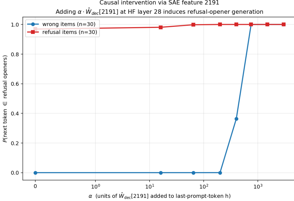
Figure 12: Causal dose-response of SAE feature 2191. On 30 ConfabQA wrong items (blue), adding \alpha \cdot \hat{W}_{dec}[2191] to the last-prompt-token hidden state at HF layer 28 induces a sharp transition between \alpha = 200 and \alpha = 750 from no refusal-opener probability to 100% of next-token mass on refusal openers (and 30/30 argmax flips). The 30 ConfabQA refusal items (red) are already saturated at \alpha = 0 .
