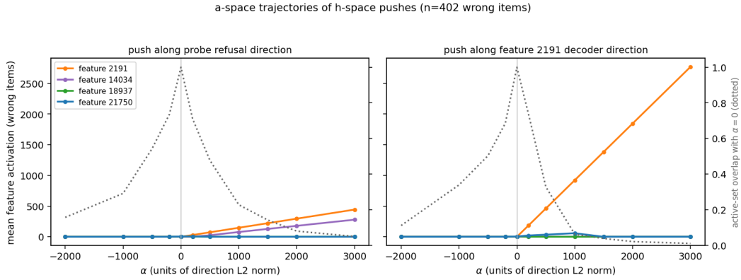
Figure 12: a-space trajectories of h-space pushes ( n = 402 wrong items). Solid lines: mean activation of the four Section 6.3 features as the layer-28 state is pushed along the probe refusal direction (left) or feature 2191’s decoder direction (right); dotted: mean overlap (Jaccard) of the active feature set with the unperturbed code. Both pushes recruit 2191 universally by \alpha = +200 and extinguish the content-cue features; large doses rewrite the code almost entirely.
