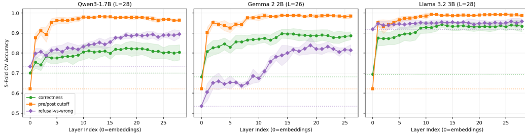
Figure 14: Comparative probing accuracy curves across Qwen3-1.7B, Gemma 2 2B, and Llama 3.2 3B (Section 7.1).
