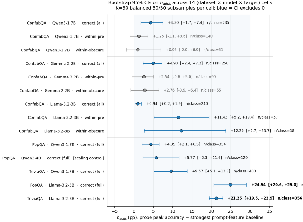
Figure 16: Forest plot of the Table 17 bootstrap 95% CIs on h_{adds} across 14 (dataset, model, target) cells. K = 30 balanced 50/50 subsamples per cell; blue = CI excludes 0. The bottom two rows are the headline positive finding: Llama 3.2 3B on PopQA / TriviaQA recovers +21–+25% over the strongest prompt-feature baseline, where Qwen3-1.7B and Qwen3-4B on the same data recover +4–+10%. The Qwen3-4B “scaling control” row rules out parameter count as the dominant driver of the cross-model gap.
