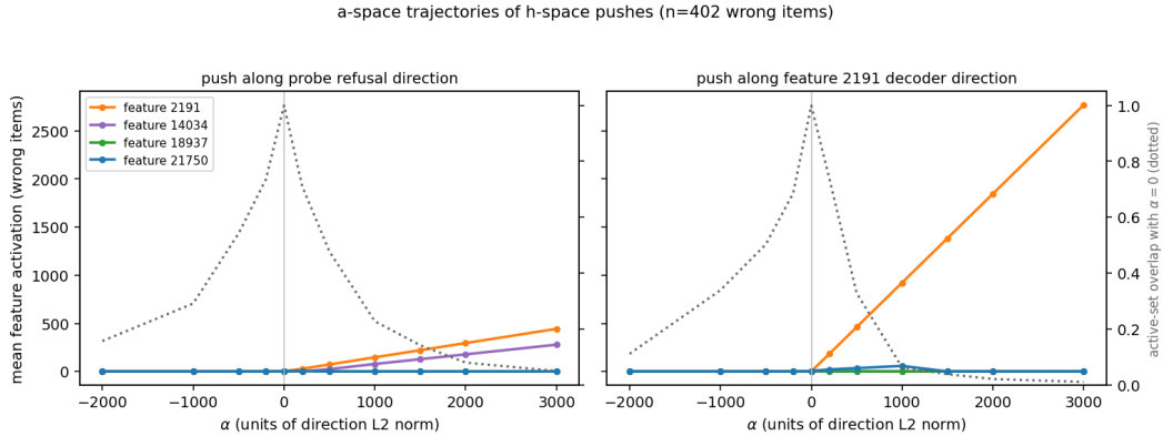
Figure 12: a-space trajectories of h-space pushes ( n = 402 wrong items). Solid lines: mean activation of the four Section 6.3 features as the layer-28 state is pushed along the probe refusal direction (left) or feature 2191’s decoder direction (right); dotted: mean overlap (Jaccard) of the active feature set with the unperturbed code. Both pushes recruit 2191 universally by \alpha = +200 and extinguish the content-cue features; large doses rewrite the code almost entirely.
