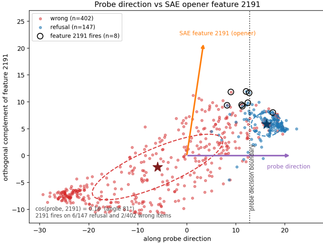
Figure 14: The plane spanned by the probe refusal direction and SAE feature 2191’s decoder vector (layer-28 refusal+wrong states, n = 549 ; stars: class centroids; dashed: per-class 1\sigma covariance ellipses). The two arrows are 81^\circ apart (cosine 0.16). The probe axis carries the class split, and its decision boundary (dotted) is again exact in this plane; the feature axis is nearly class-neutral except at its upper tail, where the eight ringed items on which 2191 actually fires sit (six refusal, two wrong: the 4.1%/0.5% hit rates of Figure 11). A rarely-firing, nearly probe-orthogonal output knob and a broad discriminative mixture share one causal channel.
