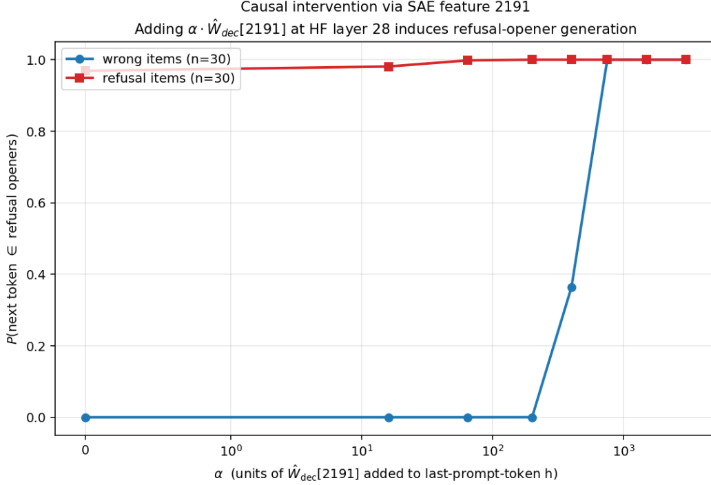
Figure 13: Causal dose-response of SAE feature 2191. On 30 ConfabQA wrong items (blue), adding \alpha \cdot \hat{W}_{\text{dec}}[2191] to the last-prompt-token hidden state at HF layer 28 induces a sharp transition between \alpha = 200 and \alpha = 750 from no refusal-opener probability to 100% of next-token mass on refusal openers (and 30/30 argmax flips). The 30 ConfabQA refusal items (red) are already saturated at \alpha = 0 .
