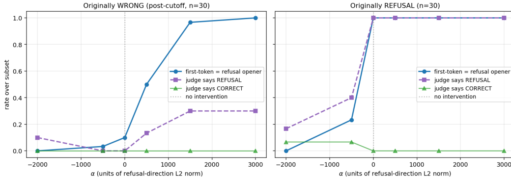
Figure 10: Causal intervention: rate over each subset as a function of \alpha . Solid blue: fraction of generations whose first generated token matches a refusal opener ( { as, As, as, 作为, ... } ). Dashed purple: fraction whose full judge label is REFUSAL. Light green: fraction labeled CORRECT (drops at high |\alpha| on the refusal subset: intervention can also break originally correct refusals into confabulations). The first-token measure changes monotonically and saturates near \alpha = \pm 1500 ; the full-judge measure changes more slowly because of autoregressive continuation dynamics.
