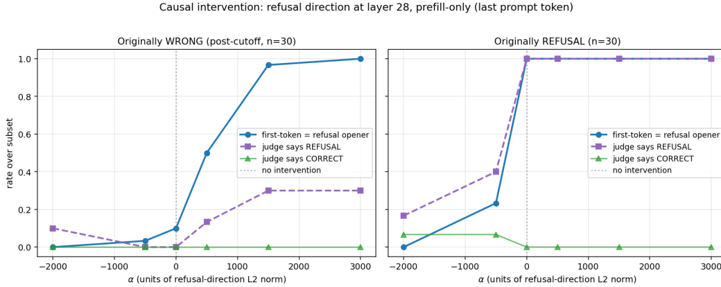
Figure 10: Causal intervention: rate over each subset as a function of \alpha . Solid blue: fraction of generations whose first generated token matches a refusal opener ( \{ \text{as, As, as, 作为, ...} \} ). Dashed purple: fraction whose full judge label is REFUSAL. Light green: fraction labeled CORRECT (drops at high |\alpha| on the refusal subset: intervention can also break originally correct refusals into confabulations). The first-token measure changes monotonically and saturates near \alpha = \pm 1500 ; the full-judge measure changes more slowly because of autoregressive continuation dynamics.
