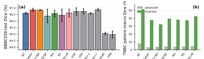
Fig. 1. (a) BBBC039 Dice across all matched models (mean±seed SD; truncated axis). (b) Patient-macro TNBC transfer before and after fixed grayscale inversion.
