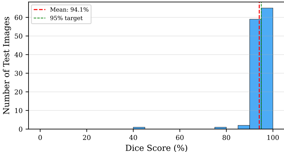
Distribution of Per-Image Dice Scores (Proposed)
