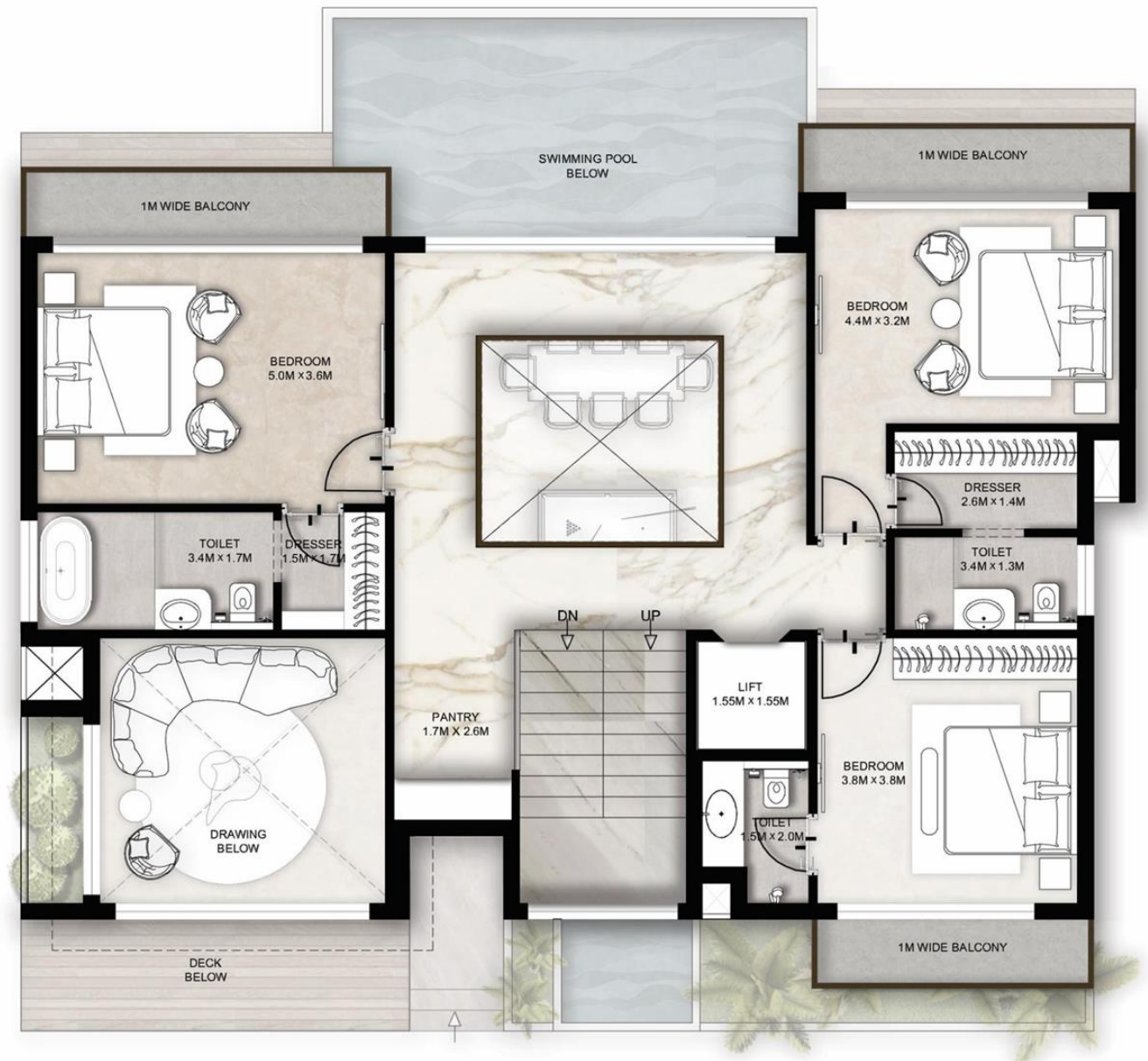
VILLA 2 FIRST FLOOR
