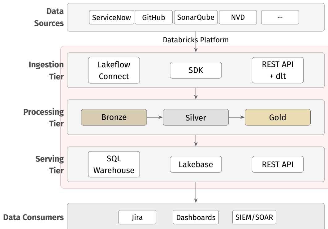
Figure 2.1 Component Design
