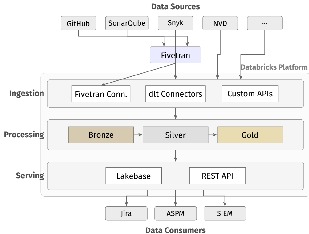
Figure 3.1 Pipeline Architecture
