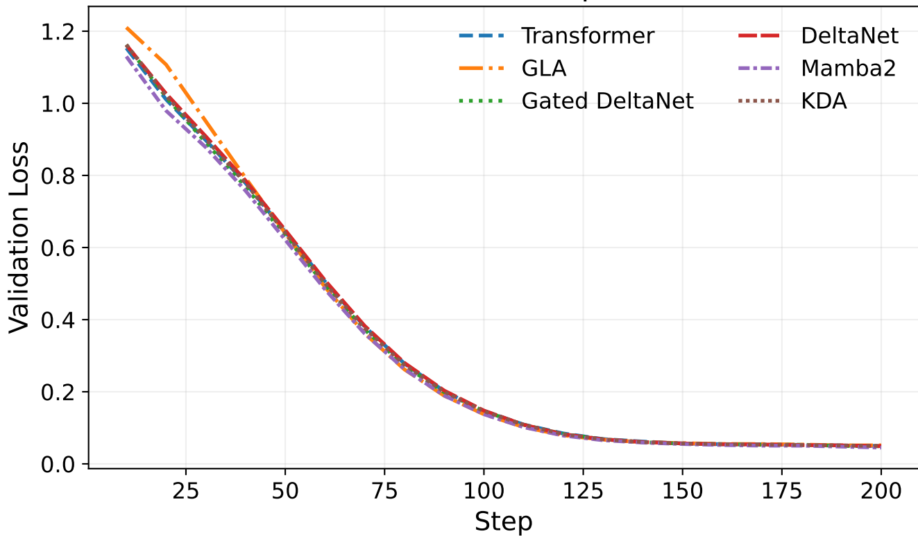
Evaluation Loss (Steps 1-200)
