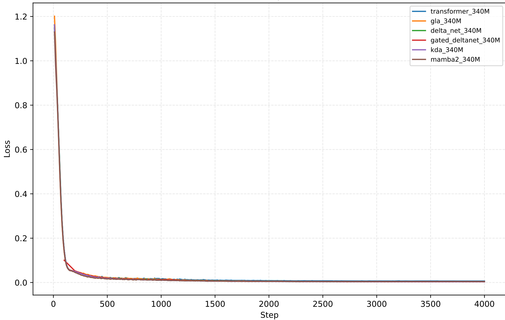
Eval Loss (Steps 1-4000)
