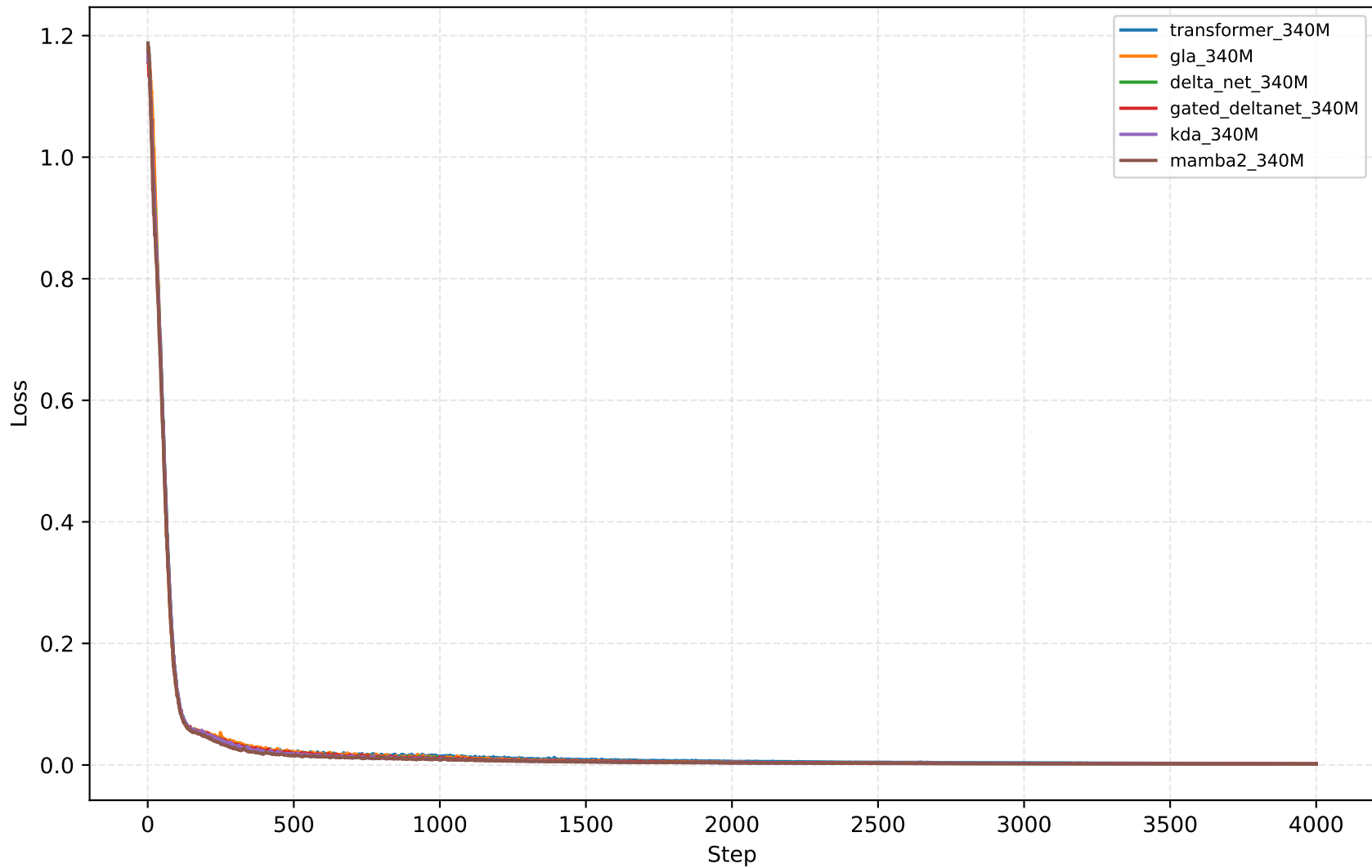
Training Loss (Steps 1-4000)
