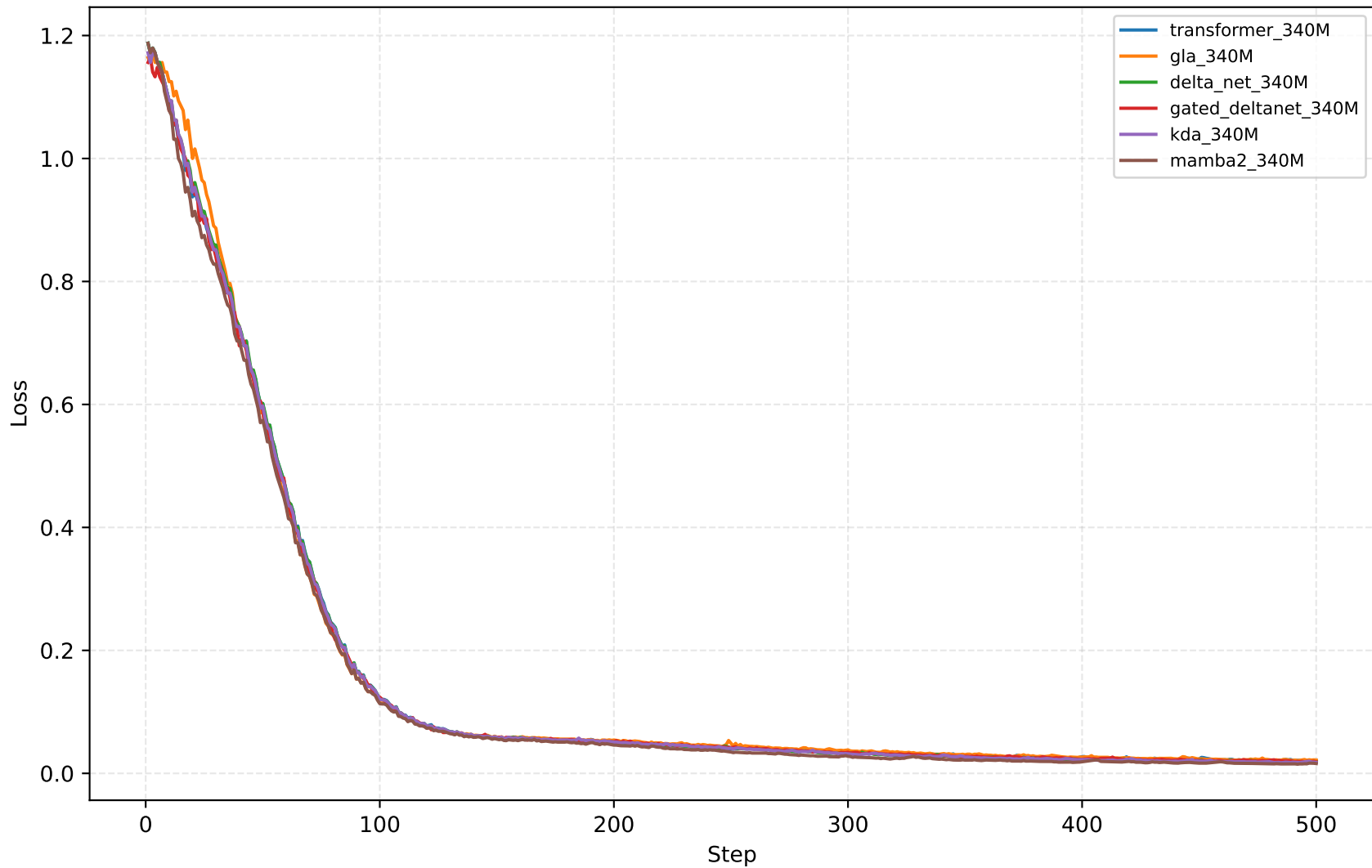
Training Loss (Steps 1-500)
