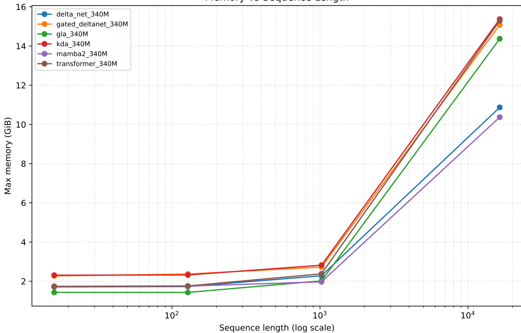
Memory vs Sequence Length
