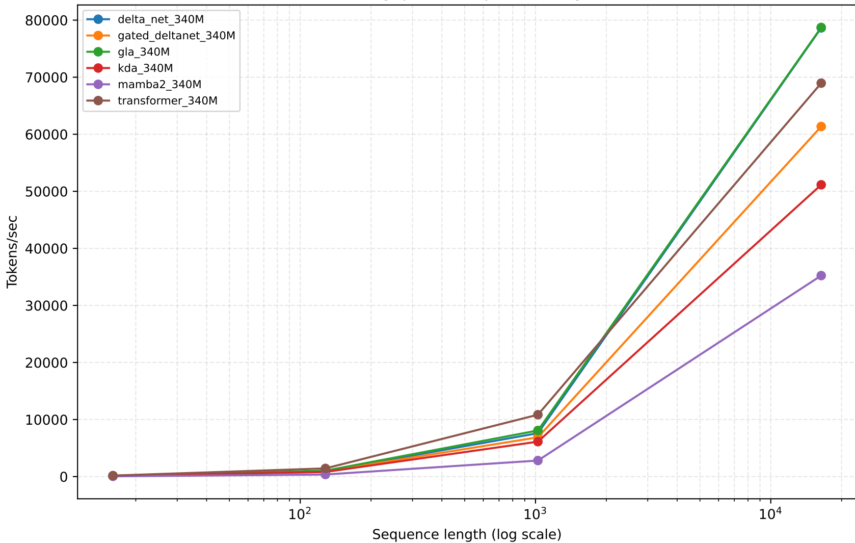
Throughput vs Sequence Length
