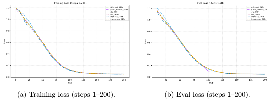
Fig. 2: Training and evaluation loss on HGT over the first 200 steps for Transformer, GLA, DeltaNet, Gated DeltaNet, KDA, and Mamba2.
