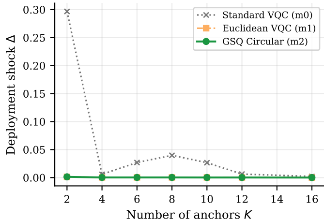
(a) Two Moons: Anchor ablation
