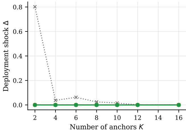
(b) MNIST 0 vs 1: Anchor ablation
