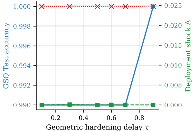
(b) MNIST 0 vs 1: Hardening delay ablation
