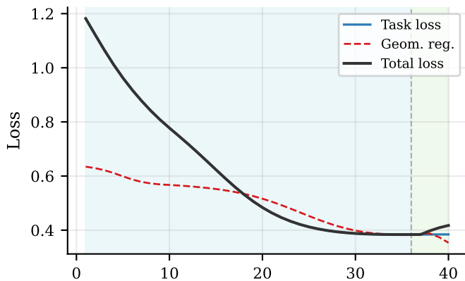
(c) MNIST 0 vs 1: Loss curves
