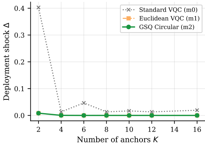
(a) Two Moons: Anchor ablation
