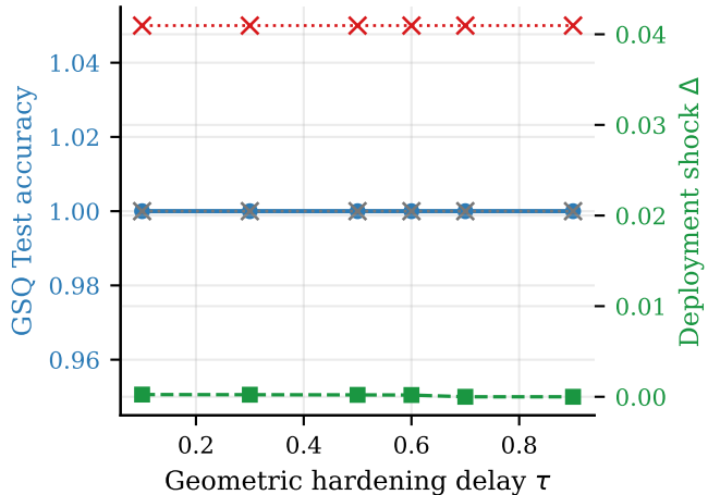
(b) MNIST 0 vs 1: Hardening delay ablation
