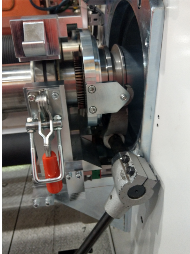
Figure 4.2-4 Example of a reel shaft located in a roll chuck with the female spline partially engaged
