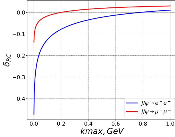
FIG. 8: Total radiative corrections as a function of k_{max} for electrons and muons.
