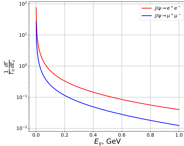
FIG. 4: Hard photon energy distribution \frac{1}{\Gamma_0} \frac{d\Gamma}{dE_\gamma} for the J/\psi \rightarrow e^+e^- and J/\psi \rightarrow \mu^+\mu^- decay modes.
