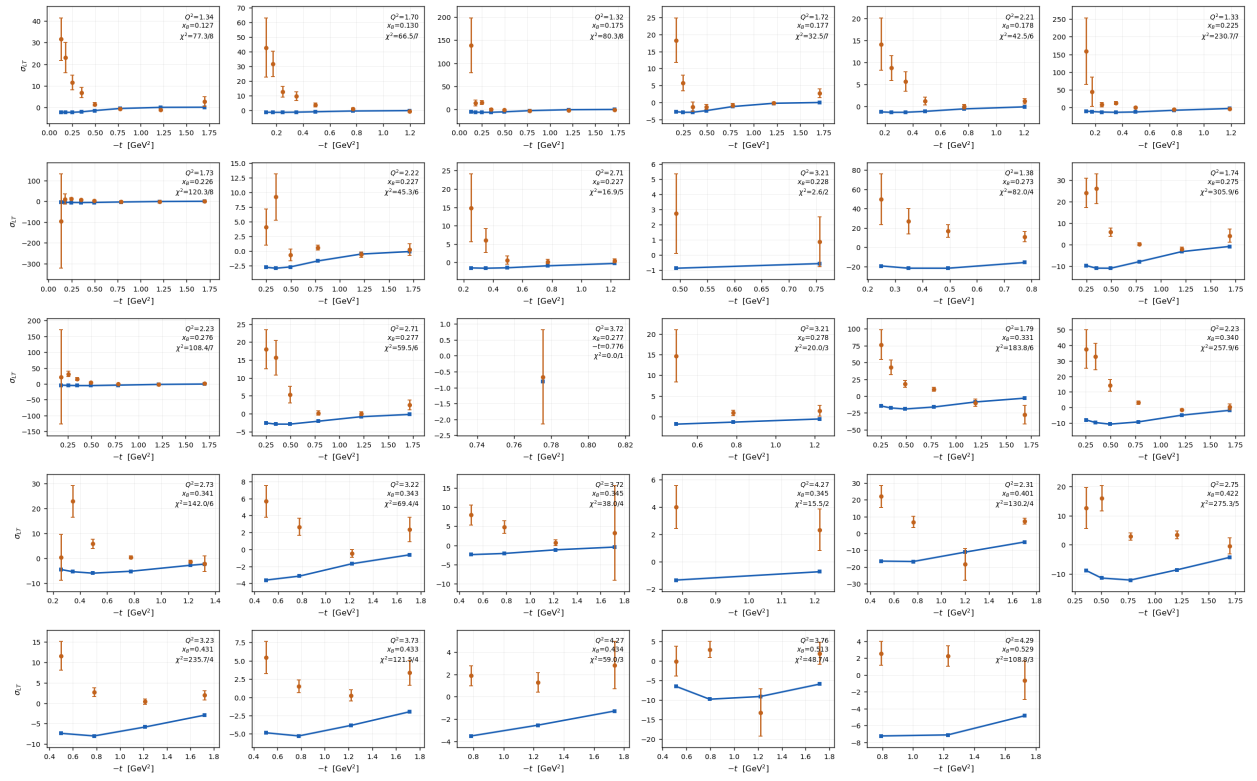
Figure 18: CLAS12, \sigma_{LT} , blind: 20.4 per point. This is the clearest single picture of the model's failure in \sigma_{LT} .
