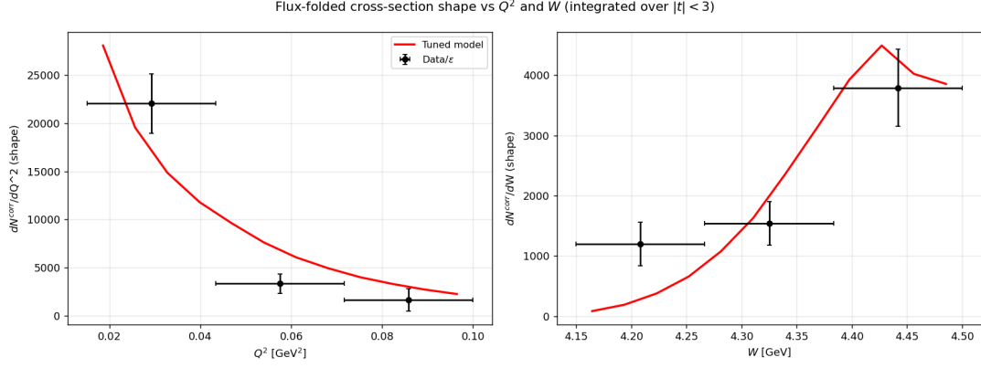
Figure 4: Cross-section shape vs Q^2 and W , integrated over |t| < 3 \text{ GeV}^2 .
