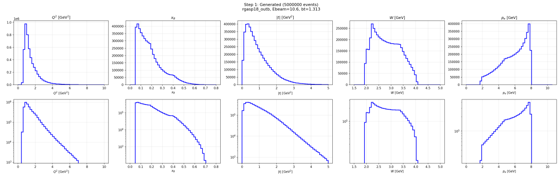
Figure 39: Generated kinematics for RGA Spring 2018, outbending.
