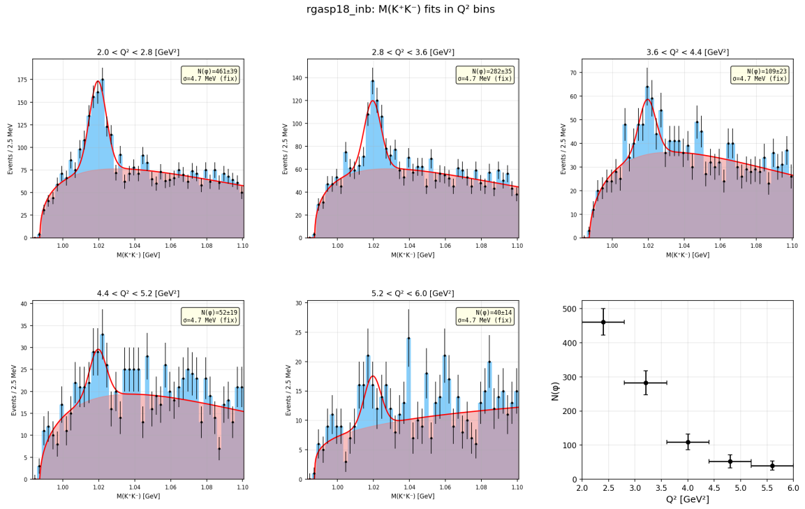
Figure 14: M(K^+K^-) fits in bins of Q^2 for RGA Spring 2018, inbending.
