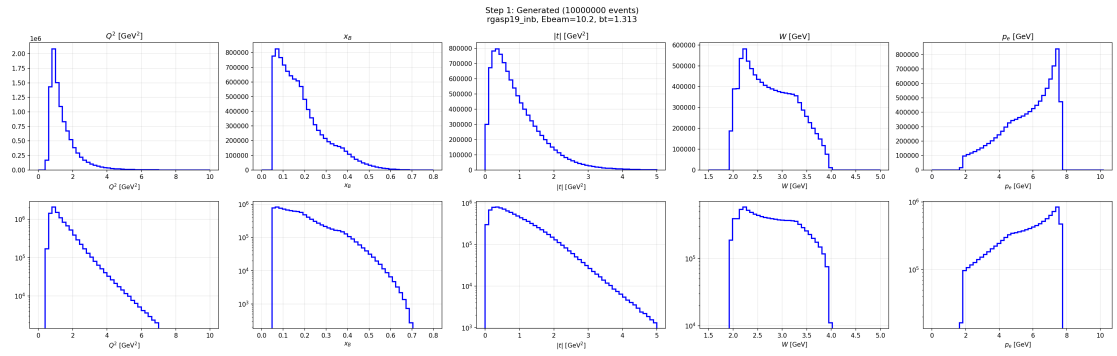
Figure 40: Generated kinematics for RGA Spring 2019, inbending.
