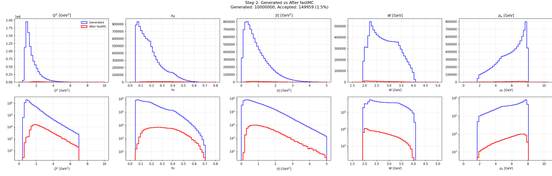
Figure 1: Generated vs. accepted distributions after fast MC for RGA Fall 2018, inbending.
