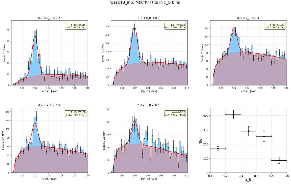
Figure 16: M(K^+K^-) fits in bins of x_B for RGA Spring 2018, inbending.
