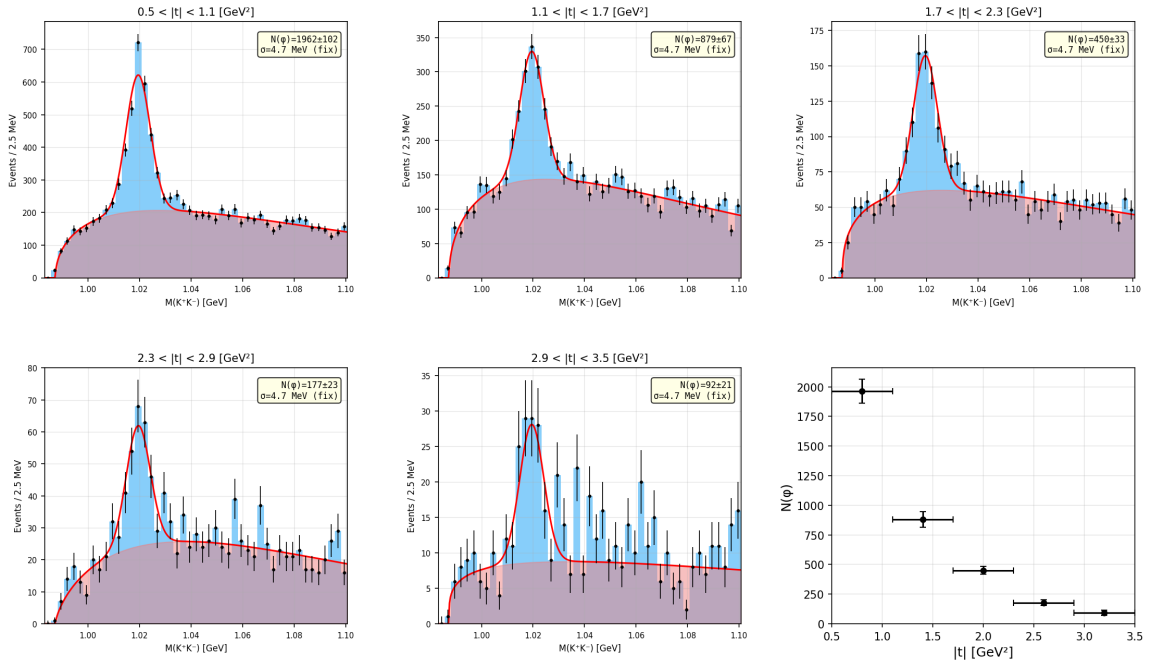
Figure 11: M(K^+K^-) fits in bins of |t| for RGA Fall 2018, outbending.
