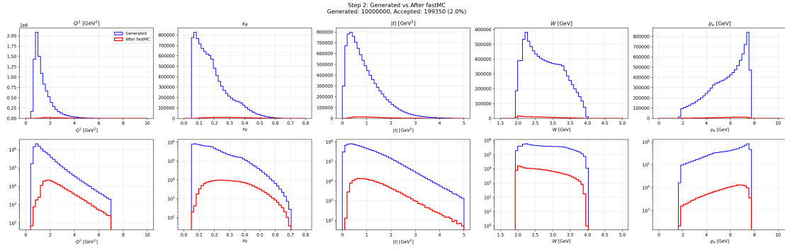
Figure 5: Generated vs. accepted distributions after fast MC for RGA Spring 2019, in-bending.
