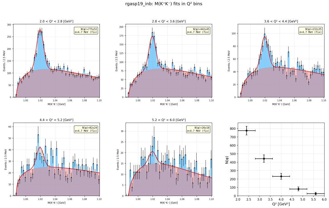
Figure 22: M(K^+K^-) fits in bins of Q^2 for RGA Spring 2019, inbending.
