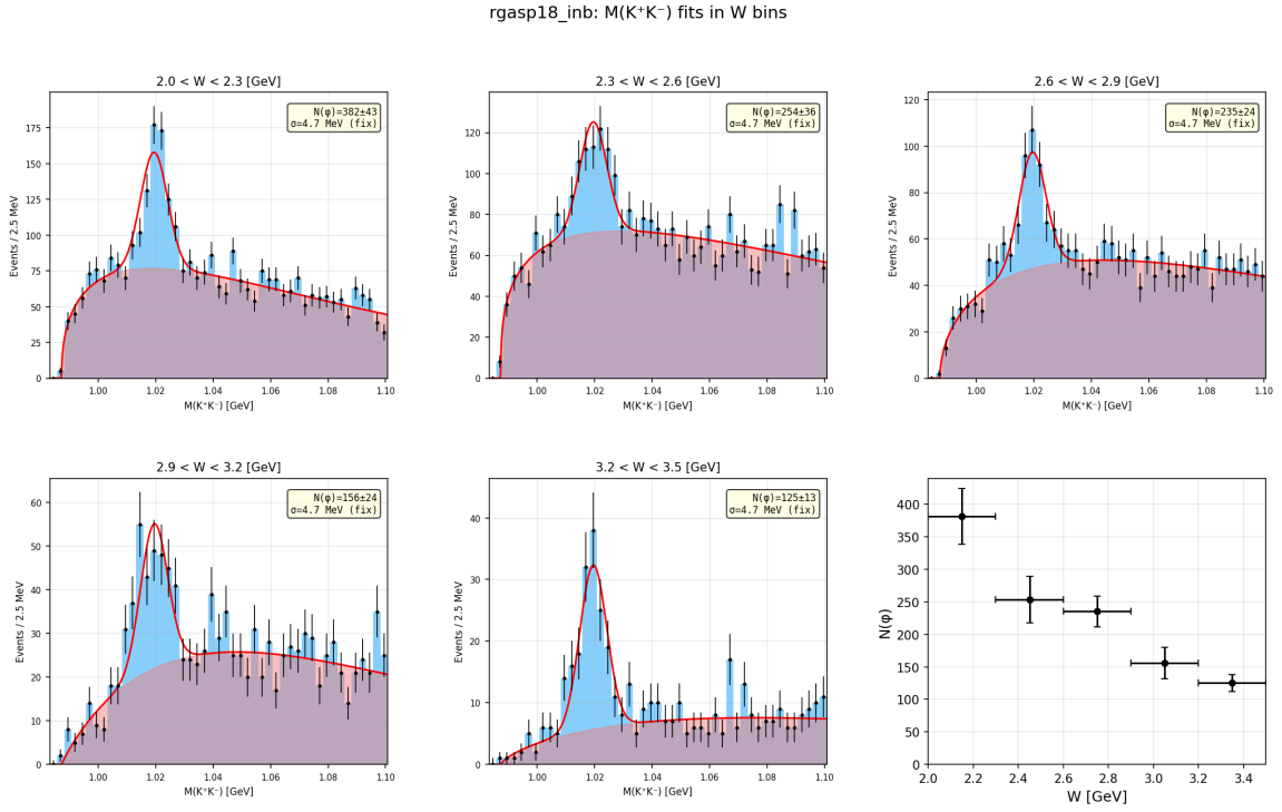
Figure 17: M(K^+K^-) fits in bins of W for RGA Spring 2018, inbending.
