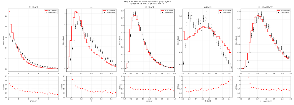
Figure 44: MC vs. data kinematic comparison for RGA Spring 2018, outbending.
