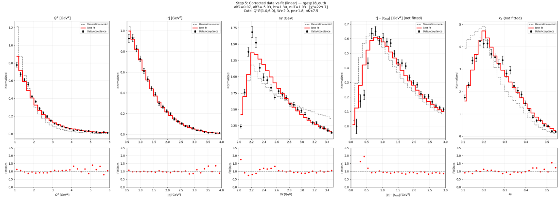
Figure 34: Pipeline step 5: acceptance-corrected fit for RGA Spring 2018, outbending (raw counts, not M(KK) signal extraction).
