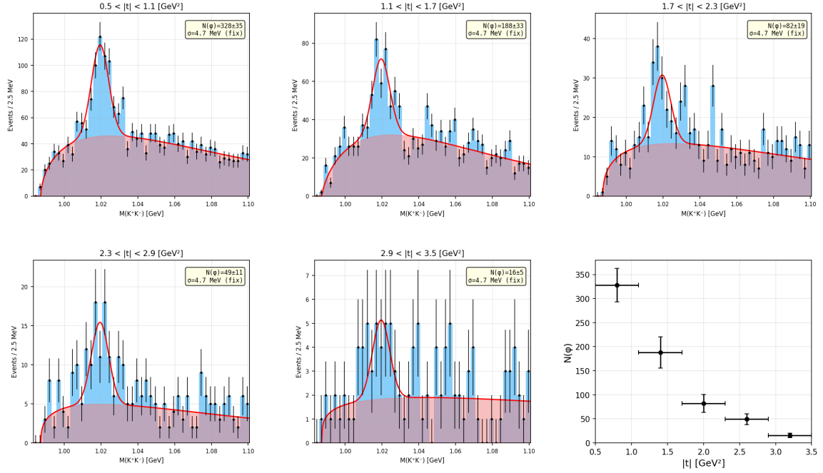
Figure 19: M(K^+K^-) fits in bins of |t| for RGA Spring 2018, outbending.
