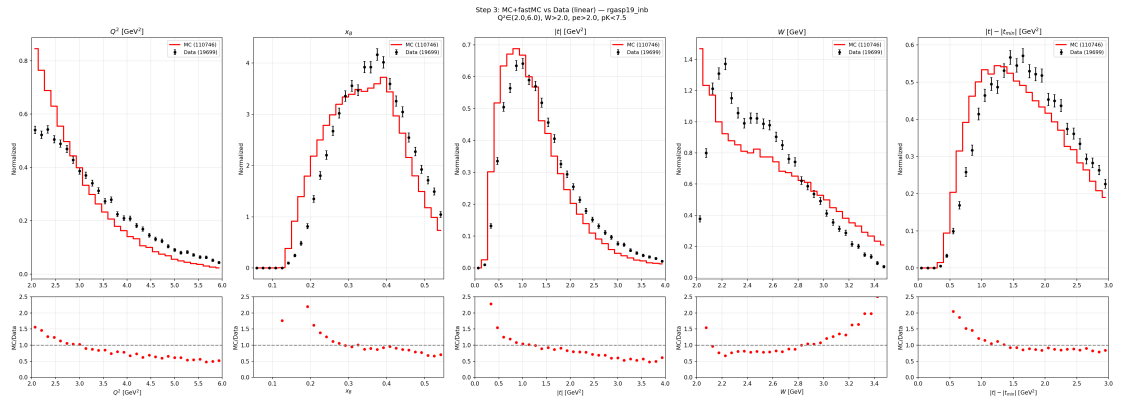
Figure 45: MC vs. data kinematic comparison for RGA Spring 2019, inbending.
