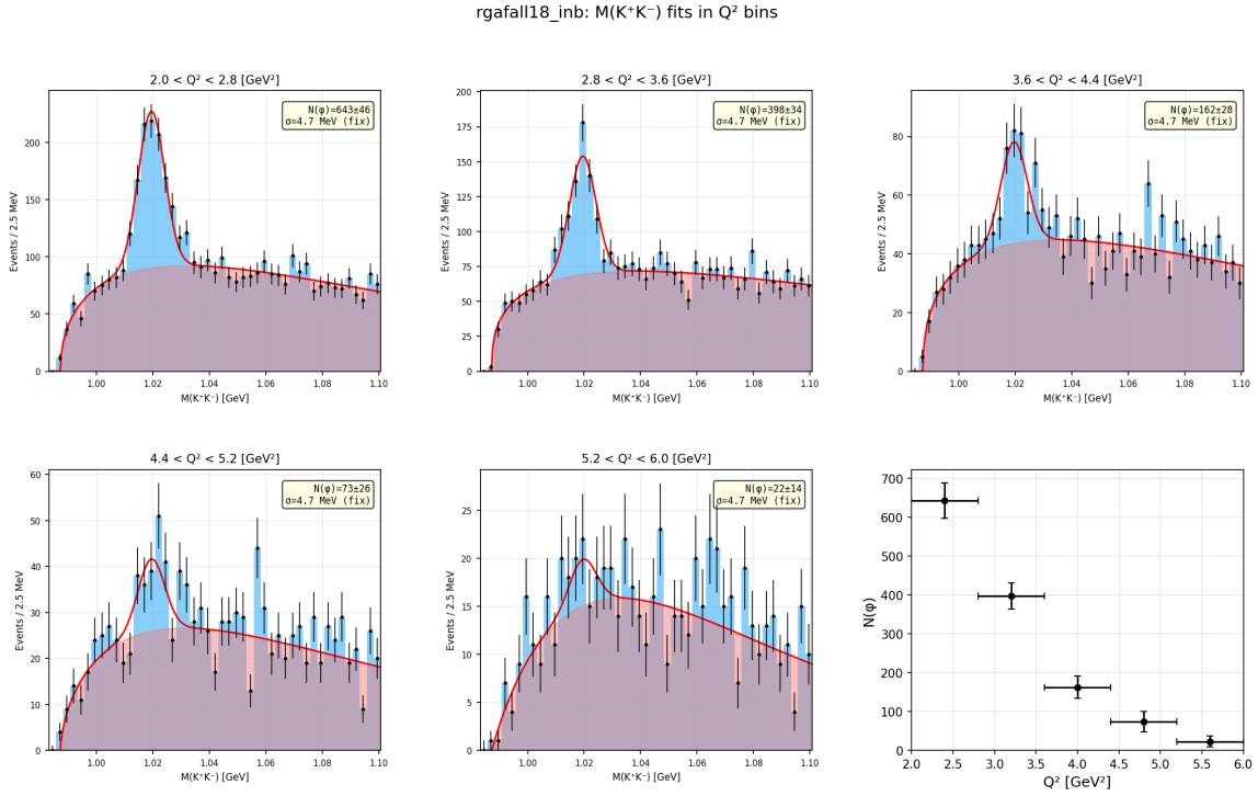
Figure 6: M(K^+K^-) fits in bins of Q^2 for RGA Fall 2018, inbending.
