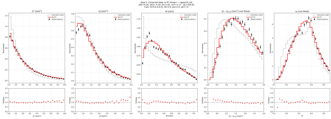
Figure 35: Pipeline step 5: acceptance-corrected fit for RGA Spring 2019, inbending (raw counts, not M(KK) signal extraction).
