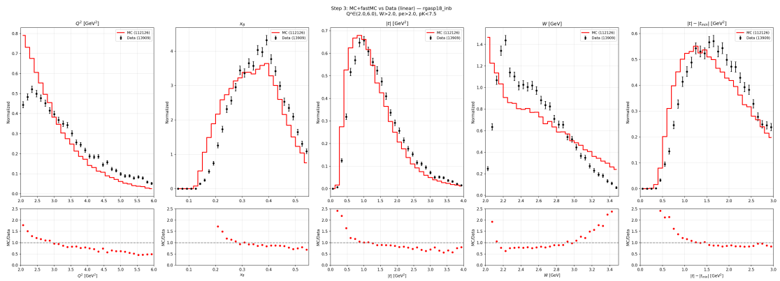
Figure 43: MC vs. data kinematic comparison for RGA Spring 2018, inbending.
