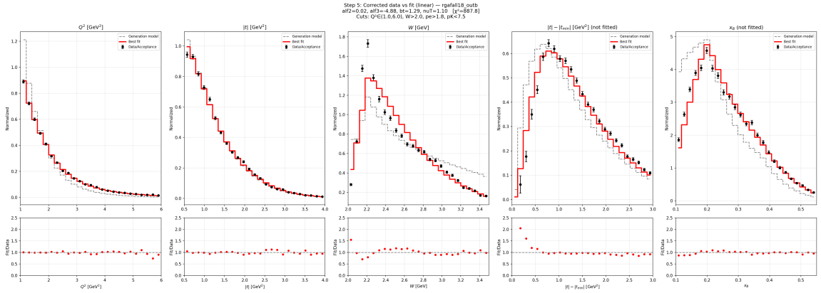
Figure 32: Pipeline step 5: acceptance-corrected fit for RGA Fall 2018, outbending (raw counts, not M(KK) signal extraction).
