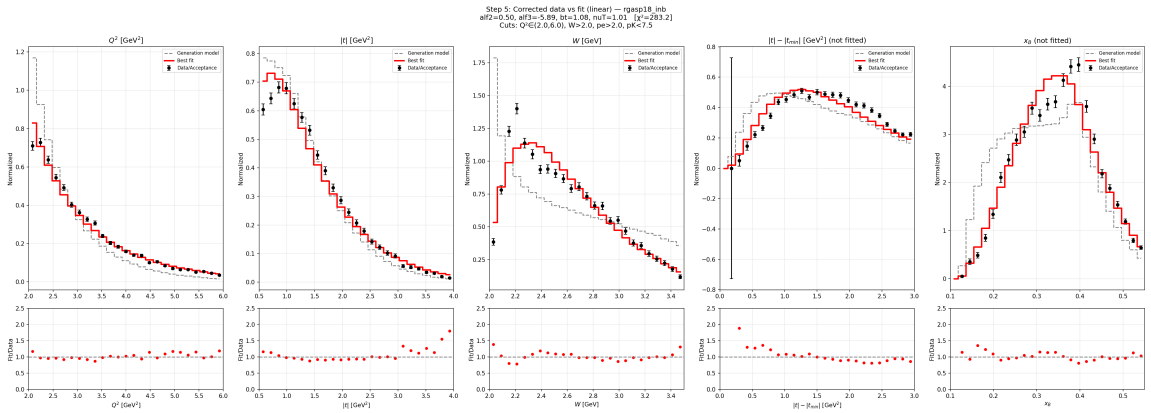
Figure 33: Pipeline step 5: acceptance-corrected fit for RGA Spring 2018, inbending (raw counts, not M(KK) signal extraction).
