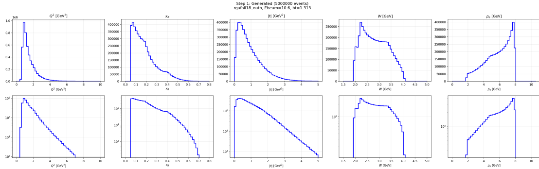
Figure 37: Generated kinematics for RGA Fall 2018, outbending.
