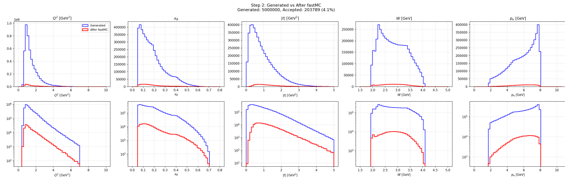
Figure 2: Generated vs. accepted distributions after fast MC for RGA Fall 2018, outbending.
