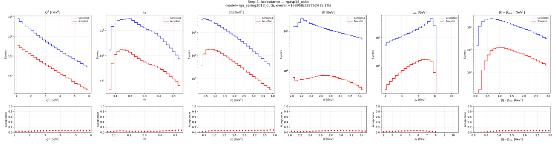
Figure 49: Acceptance maps for RGA Spring 2018, outbending.
