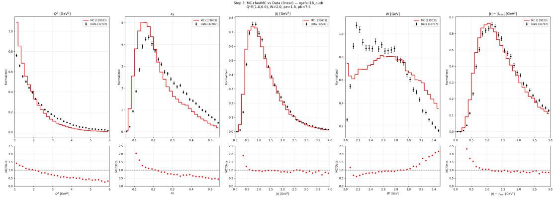
Figure 42: MC vs. data kinematic comparison for RGA Fall 2018, outbending.
