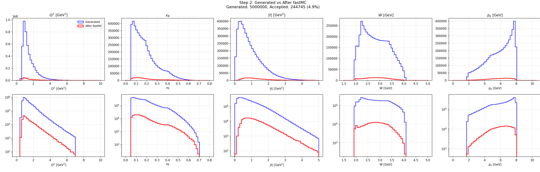
Figure 4: Generated vs. accepted distributions after fast MC for RGA Spring 2018, out-bending.
