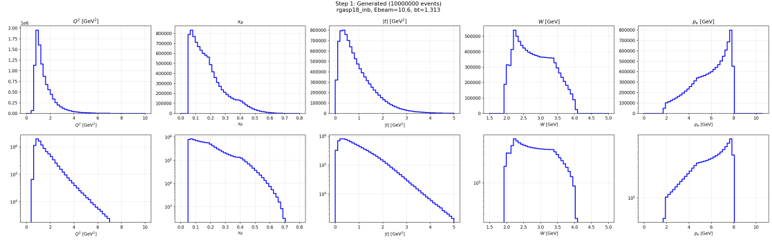
Figure 38: Generated kinematics for RGA Spring 2018, inbending.
