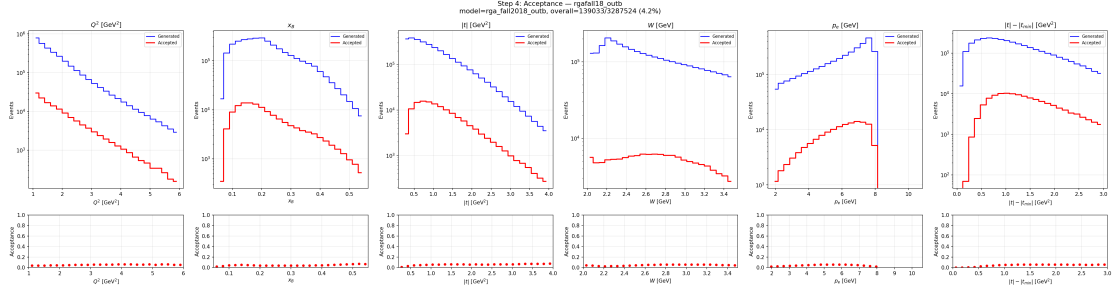
Figure 47: Acceptance maps for RGA Fall 2018, outbending.
