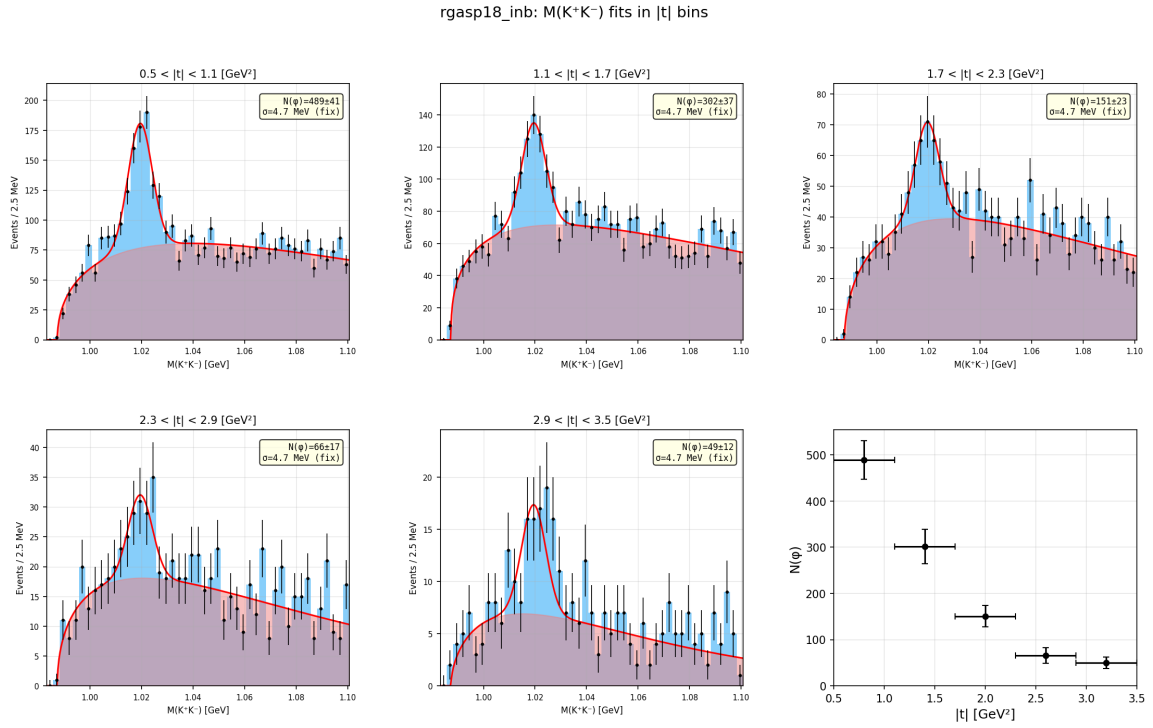
Figure 15: M(K^+K^-) fits in bins of |t| for RGA Spring 2018, inbending.
