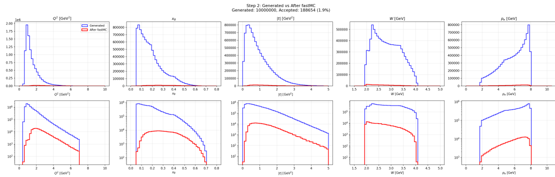
Figure 3: Generated vs. accepted distributions after fast MC for RGA Spring 2018, inbending.
