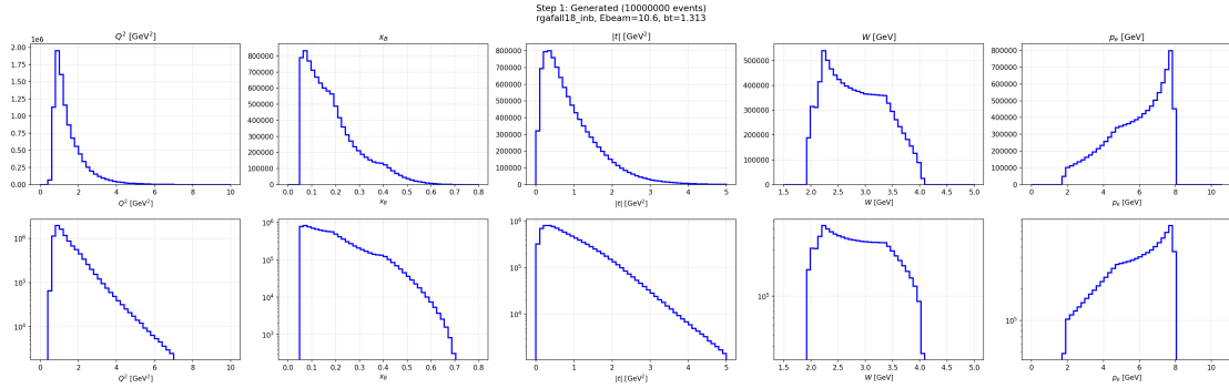
Figure 36: Generated kinematics for RGA Fall 2018, inbending.
