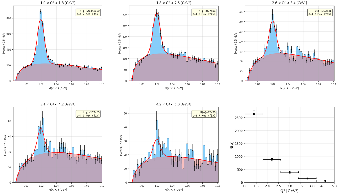
Figure 10: M(K^+K^-) fits in bins of Q^2 for RGA Fall 2018, outbending.
