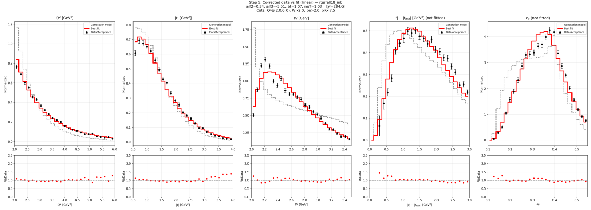
Figure 31: Pipeline step 5: acceptance-corrected fit for RGA Fall 2018, inbending (raw counts, not M(KK) signal extraction).
