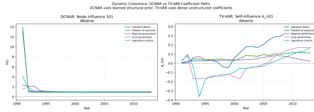
Figure 5: Dynamic coherence: DCNAR node-influence paths \lambda(t) (left) versus TV-VAR self-influence coefficients A_{ii}(t) (right) for Albania. DCNAR uses the learned structural prior; TV-VAR uses dense, unstructured coefficients. DCNAR paths stabilize after the early-1990s transition, whereas TV-VAR coefficients remain comparatively erratic.
