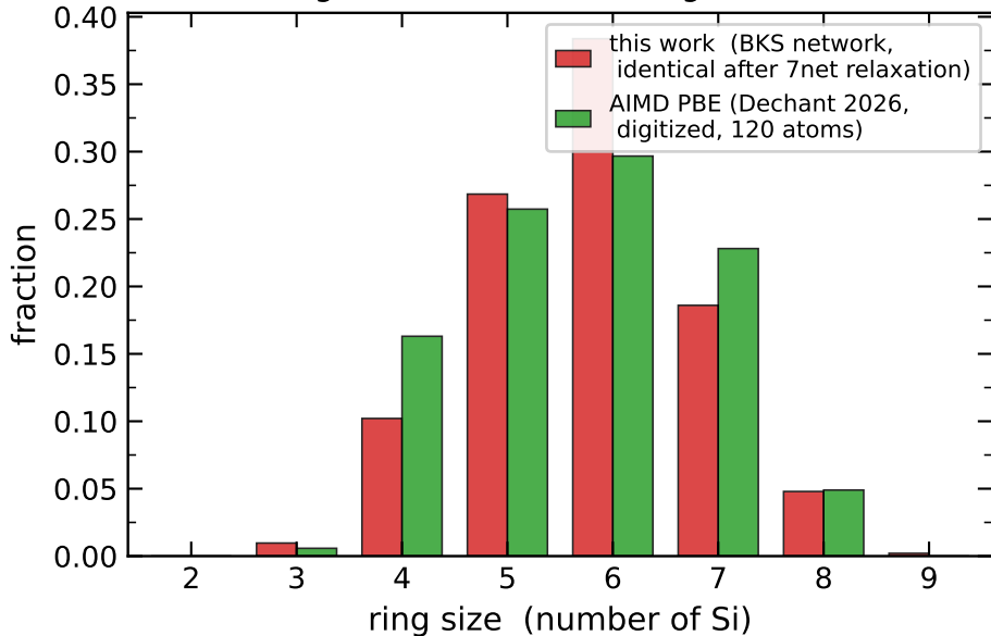
Ring size distribution (King criterion)
