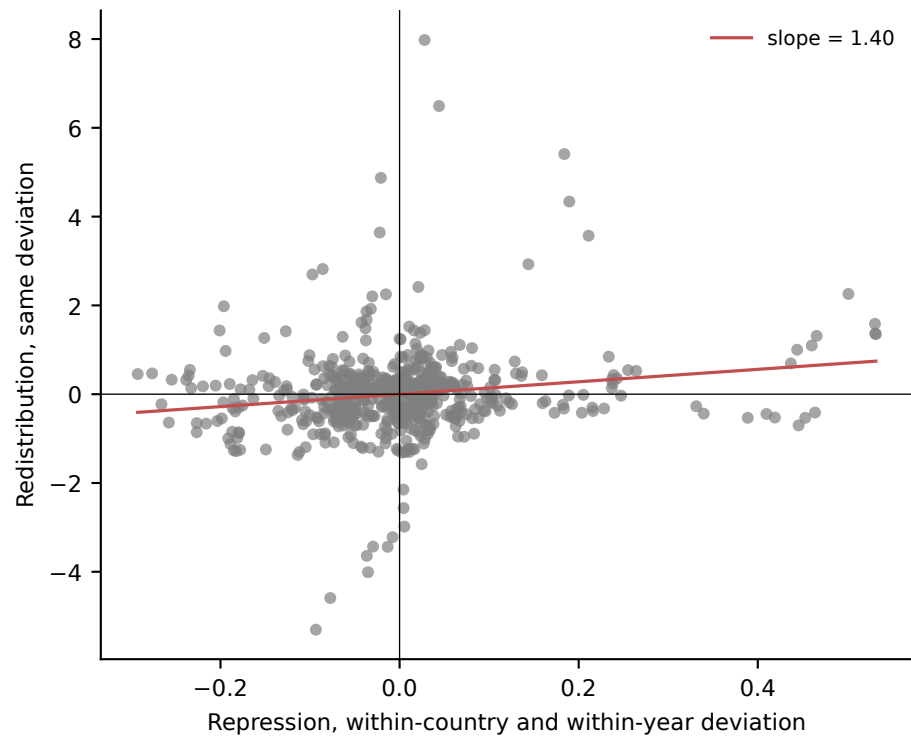
(b) Exact country and year fixed-effect residuals
