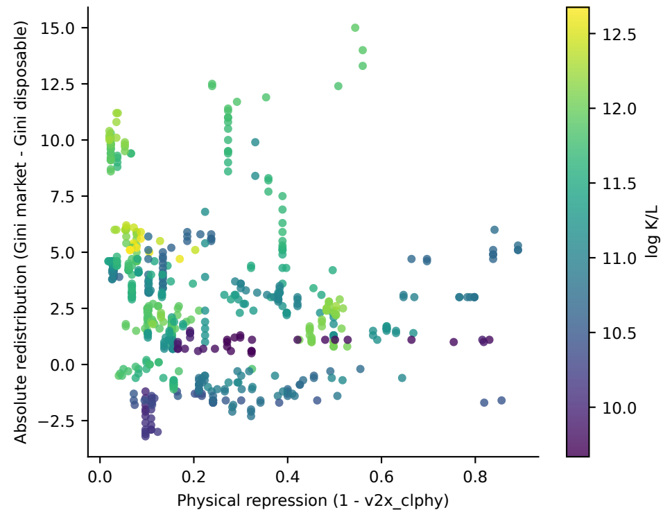
(a) Country-years 1990-2024, colour = log K/L
