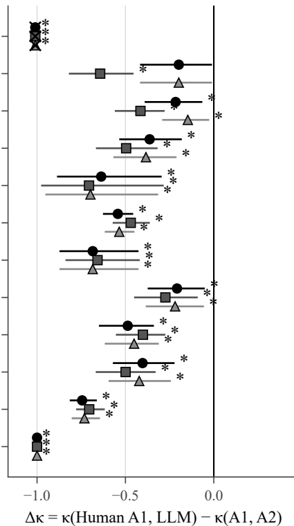
Mistral 7B
