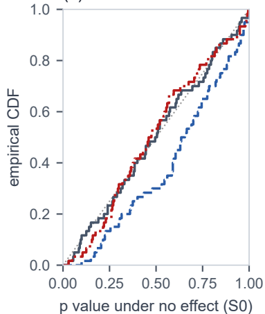
(a) Calibration under S0
