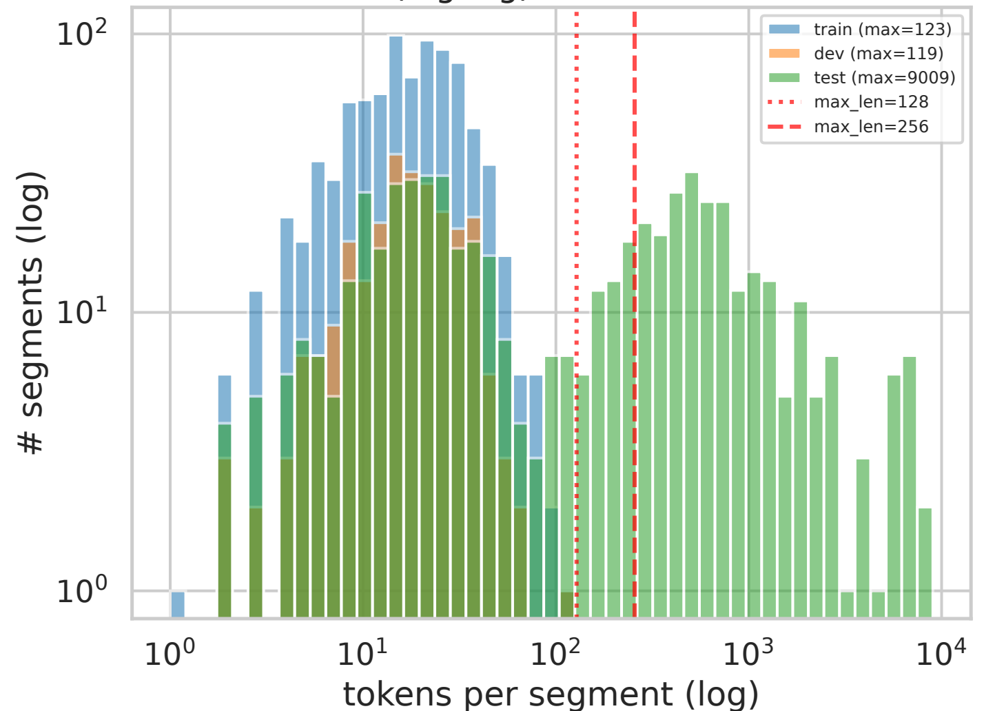
Full distribution (log-log) — reveals test-set outliers
