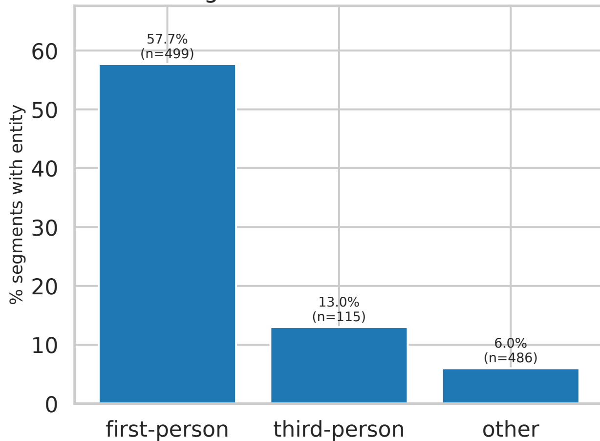
Segment-level classification
