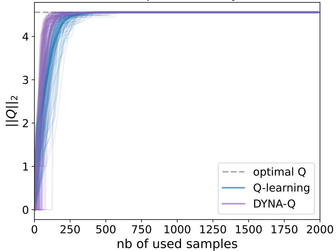
Sample efficiency
