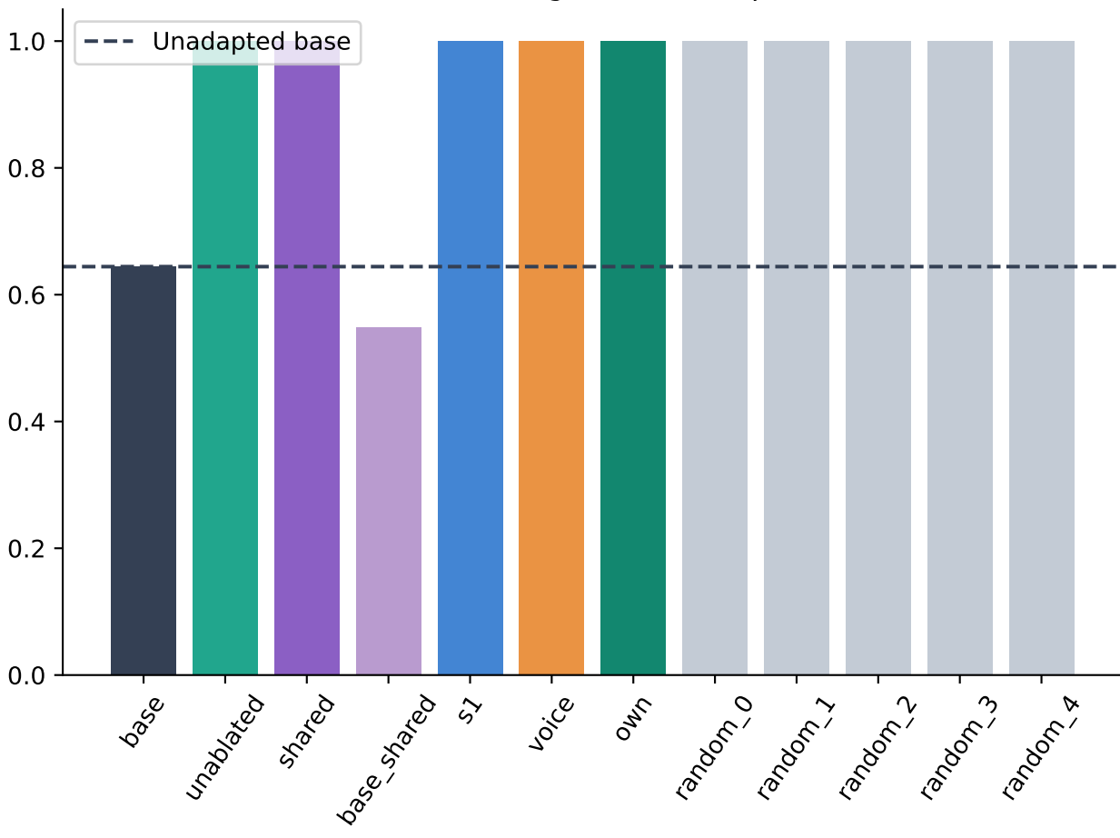
Rule following on held-out pairs
