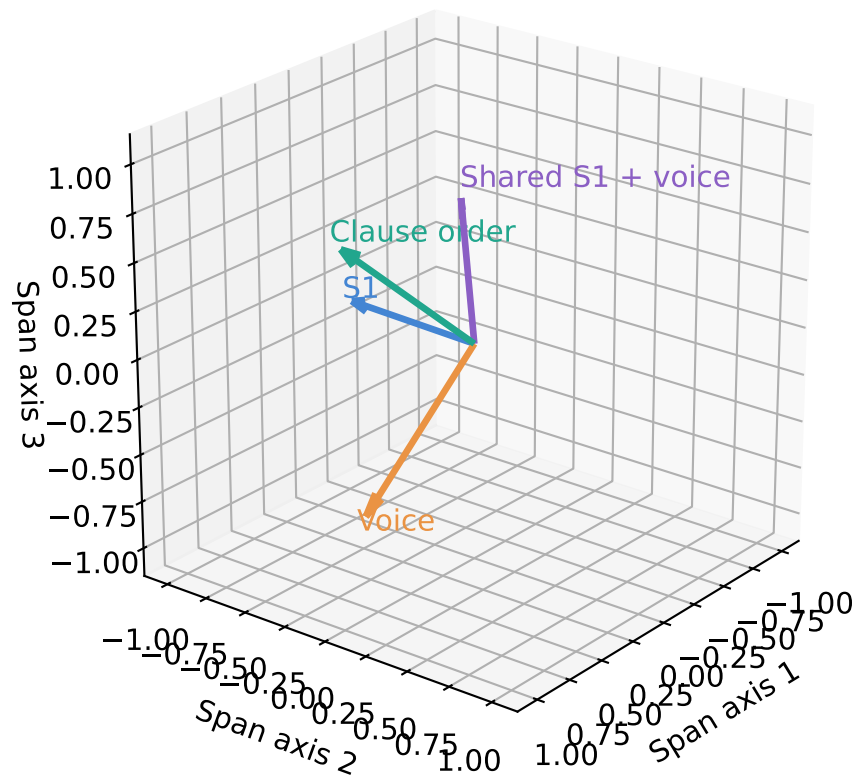
Residual directions at layer 14
