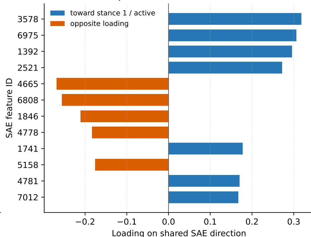
C Top 12 shared-direction features
