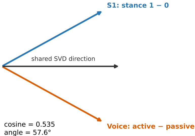
A Task-mean alignment
