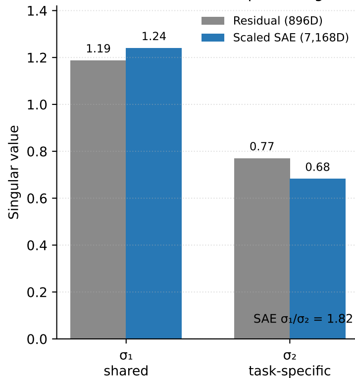
B Shared versus task-specific signal
