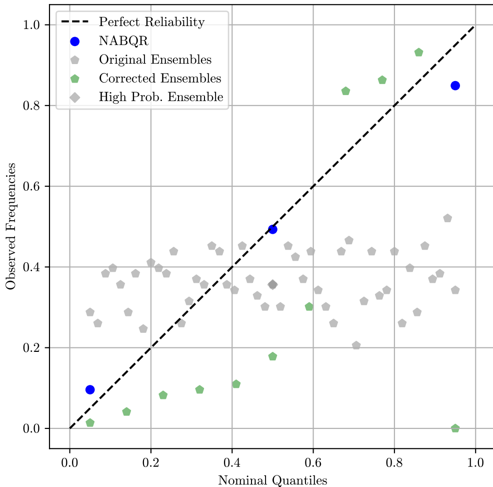
Reliability Plot for NABQR-TEST
